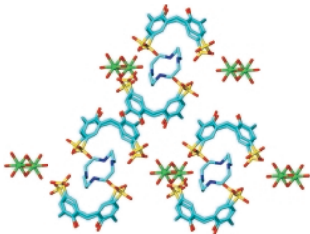
Fig. 6 Crystal structure of [\text{Cr}_2(\text{OH})_2(\text{H}_2\text{O})_8][\text{H}_4(\text{cyclam})]\text{C}\{p\text{-sulfonatocalix[4]arene(4-)}\}_2\cdot 6\text{H}_2\text{O} (waters and hydrogens omitted for clarity) showing packing of superanion capsules with a bilayer arrangement of calixarenes and [\text{Cr}_2(\text{OH})_2(\text{H}_2\text{O})_8]^{4+} cations situated at the hydrophilic equator of the capsules. 30
