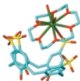
Fig. 11 The 'ferris wheel' assembly [\{\text{La}(\text{18-crown-6})(\text{OH}_2)_3\} \cap \{(p\text{-sulfonatocalix[4]arene}(4-)) + 2\text{H}^+\}]^+ ; hydrated crystals are isolated as the chloride salt. 43
