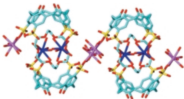
Fig. 9 Capsule formation in the complex [\{18\text{-crown-6}\}C\{(Y(H_2O)_7)_{1.33}(p\text{-sulfonatocalix[4]arene(4-))}_2\}]^+ (from the crystal structure). There are two types of [Y(H_2O)_7]^{3+} moiety, one with the Y shown in dark blue is fully ordered and positioned towards the centre of the capsule, the other, with the Y centre in pink, is disordered with a 1/3 occupancy and points away from the capsule core. Eu^{3+} forms an isostructural complex. 42
