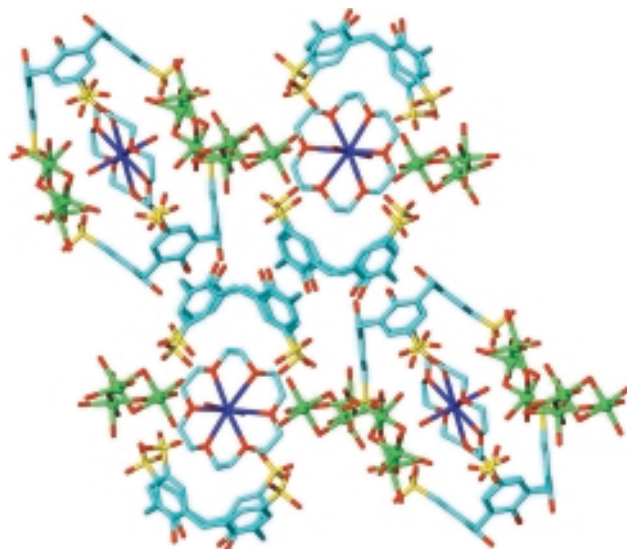
Fig. 5 Packing of superanions and partially occupied, disordered trimeric cations in [Cr_3(OH)_4(H_2O)_{10}]_2[X_3 + 11H^+] , showing the distorted bilayer arrangement of the calixarenes. 25
