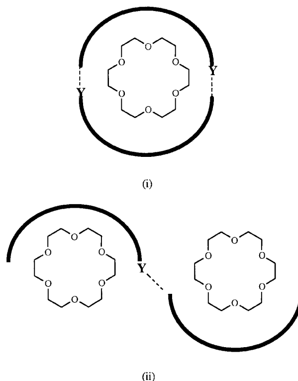
Fig. 10 Schematic representation of the hydrogen bonding modes of the capsules found in the complex [\{18\text{-crown-6}\}C\{(M(H_2O)_7)_{1.33}(p\text{-sulfonatocalix[4]arene(4-))}_2\}]^+ , M = Y or Eu (see Fig. 9): (i) the intracapsule Y-OH_2 \cdots O-S hydrogen bonding of the fully occupied M positions, (ii) the intercapsule S-type Y-OH_2 \cdots O-S hydrogen bonding of the partially occupied M positions.
