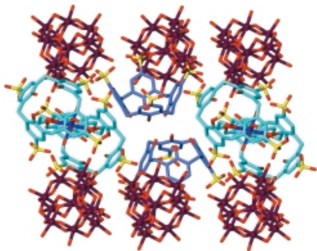
Fig. 8 Packing of the major structural components in [\text{Al}_{13}\text{O}_4(\text{OH})_{24}(\text{H}_2\text{O})_{12}]\{\text{X} + (\text{H})_{0.5}\{(\text{p-sulfonatocalix}[4]\text{arene}(4-))(\text{H}^+)_{\text{y}}\}(\text{H}_2\text{O})_{29}\} (water molecules and hydrogens are not shown for clarity). Chains of Keggin ions (in red) are shown running across the page, chains of superanions come out of the page. Water bearing calixarenes not involved in capsule formation are highlighted in darker blue. 35
